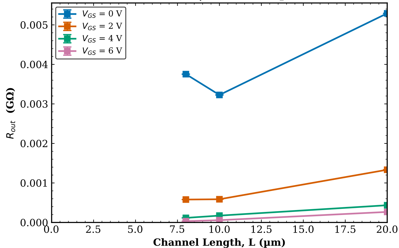
TFT1 Transistor 2 R_{out} vs L | W = 1000\text{ }\mu\text{m}
